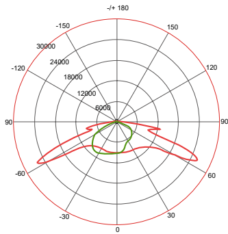
Chart 2: Isocandela Plot AVERAGE BEAM ANGLE(50%): 140.8 DEG C0/180, 165.5 C90/270, 116.1
